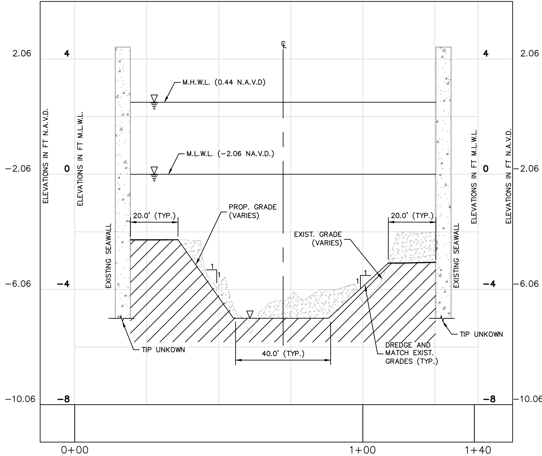
TYPICAL SECTION
